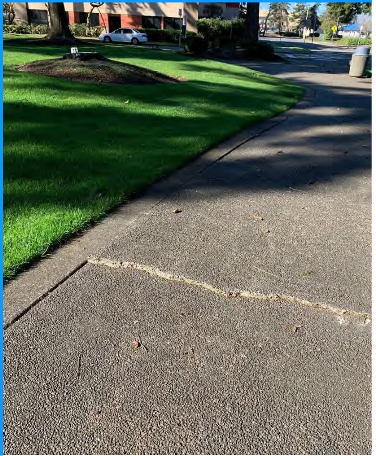
Lifted Concrete
